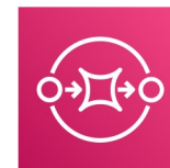
Amazon SQS
